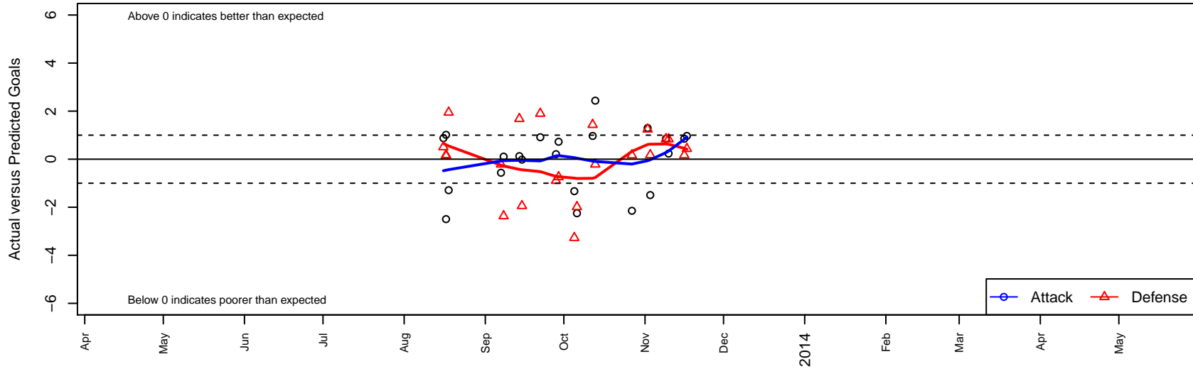
Newberg SC Dragons B99 Dots are actual minus expected GF (blue circles) and GA (red triangles). Blue line is smoothed change in attack strength. Red is smoothed change in defense strength.
